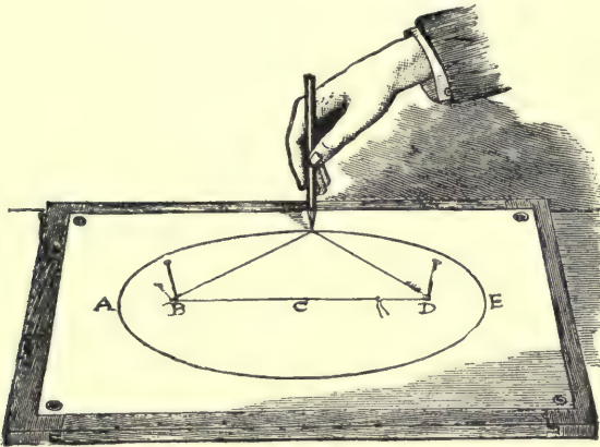
THE CONSTRUCTION OF AN ELLIPSE.
